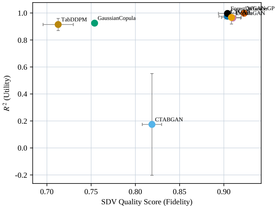
Air Quality: SDV Quality Score (Fidelity) vs R^2 (Utility)
